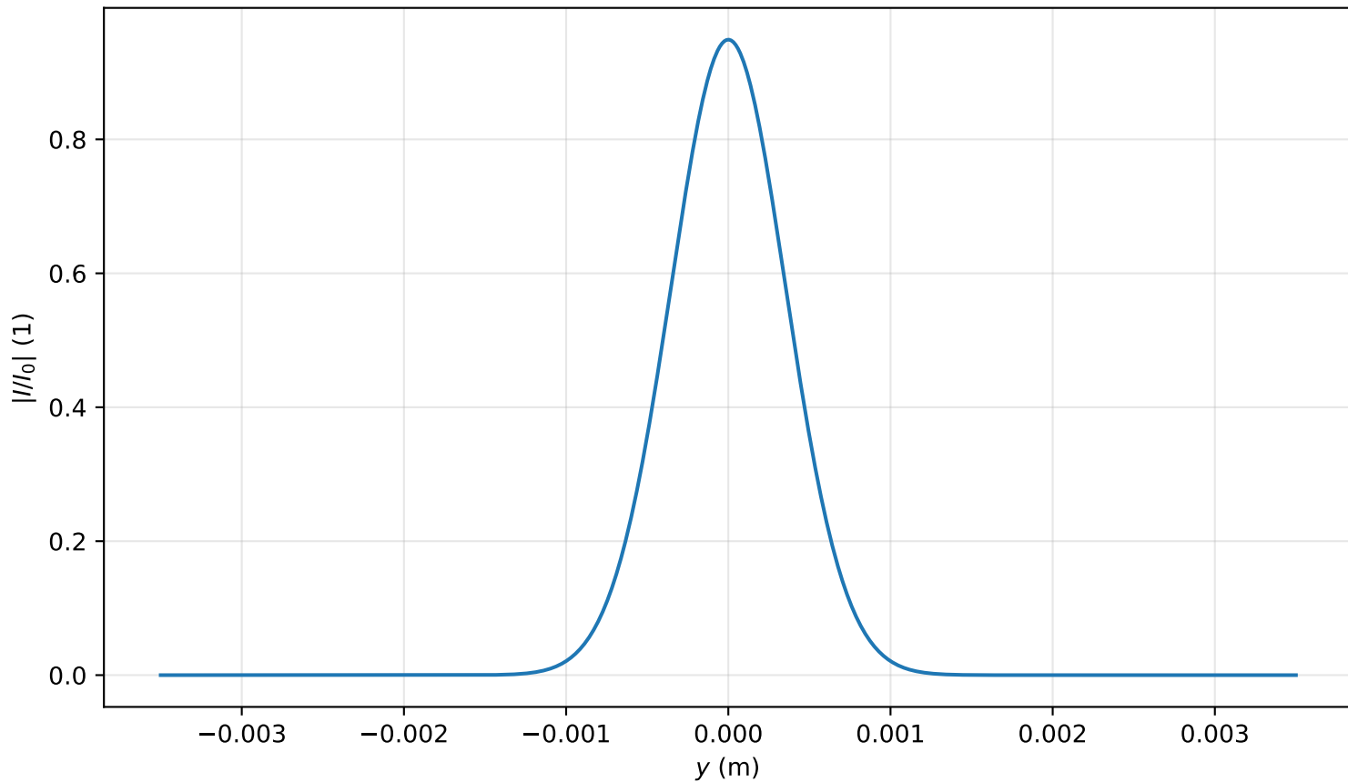
Intensity profile I(x=0, y, z=0.557)/I_0 , P_{in}=0.1P_{cr} , artificial time
